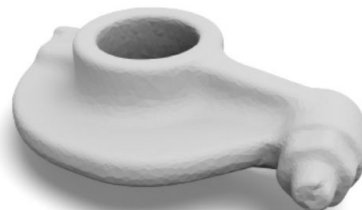
Reference
