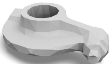
Input (rendered)
