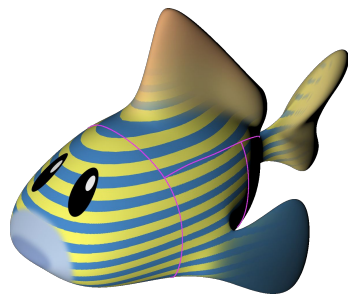
Ground Truth
