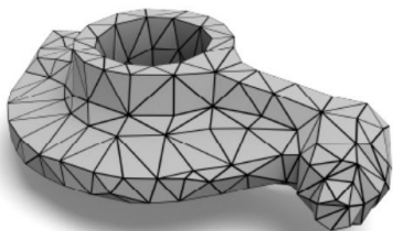
Input (wireframe)
