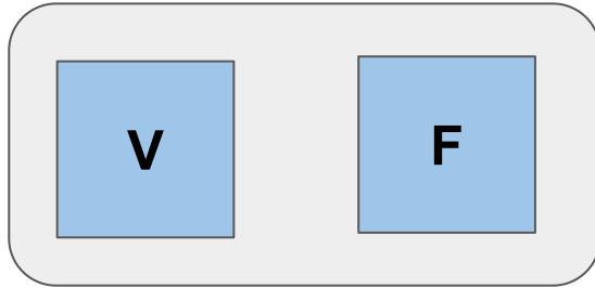
Single Resolution
