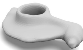
Loop
