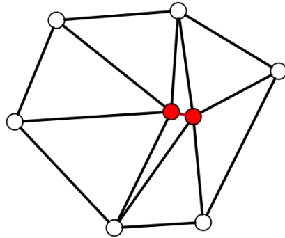
Vertex Split
