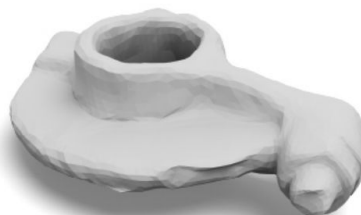
Modified Butterfly
