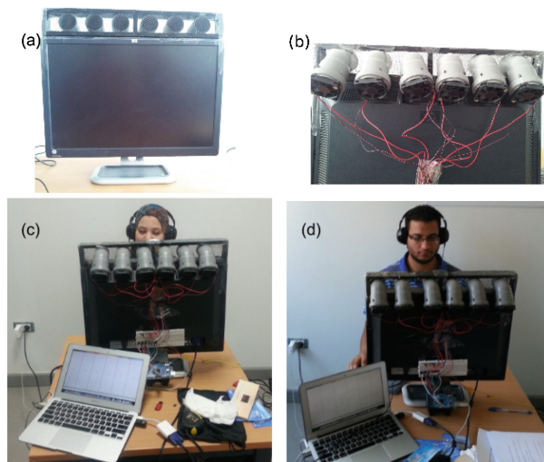
Fig. 1. (a) AirDisplay mounted on a monitor, (b) AirDisplay back view, (c) and (d) participants taking part in the experiment.
